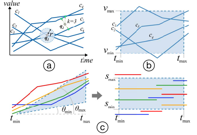
Fig. 1. Illustrations of four different lines query methods: (a) radius nearest lines (RNL) query locates lines c_1 , c_5 , and c_6 for query point \mathbf{q}_1 and radius r , where k -nearest lines (KNL) query locates lines c_3 , c_4 , and c_5 for query point \mathbf{q}_2 and k=3 ; (b) timebox query locates lines c_3 and c_4 within the box; and (c) angular query: user brushes in the time-angle domain (left) and the computation is done in the time-slope domain (right), in which continuous lines become piecewise line segments.
